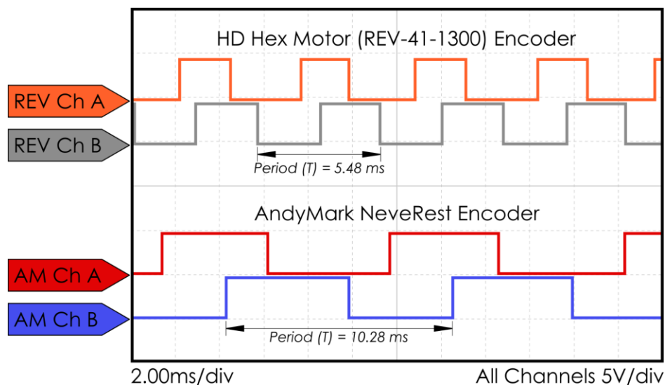
Figure 5: Encoder Output Signal Measurement with Coupled Output Shafts
