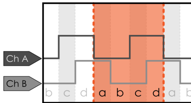
Figure 3: Encoder Cycle
